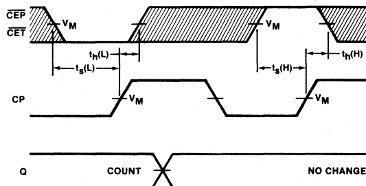
Waveform 5
