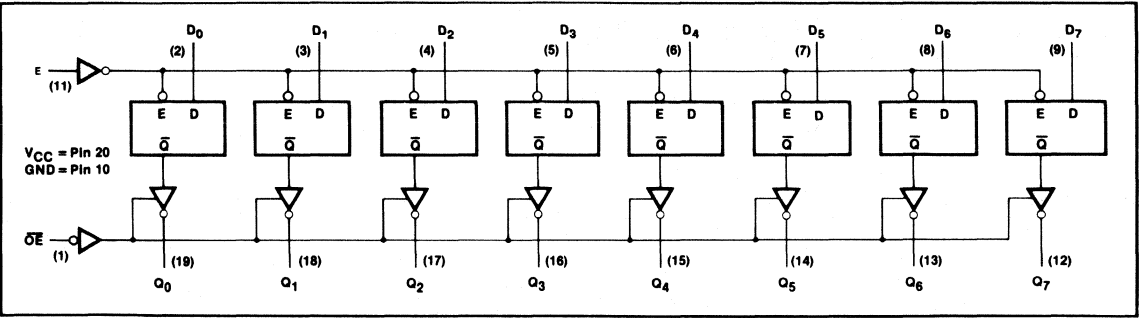
LOGIC DIAGRAM, 8TS806
