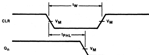
Waveform 4
