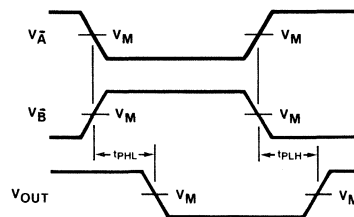
Waveform 3
