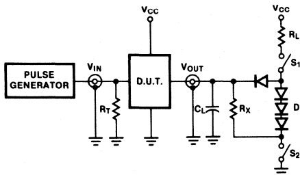
SWITCH POSITION
