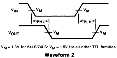
WAVEFORM FOR NON-INVERTING OUTPUTS
