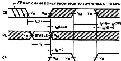
Waveform 4
