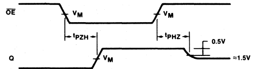
Waveform 2
