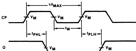
Waveform 1
