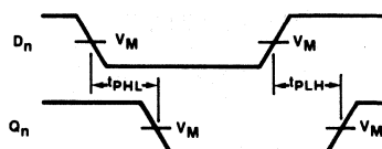
Waveform 4
