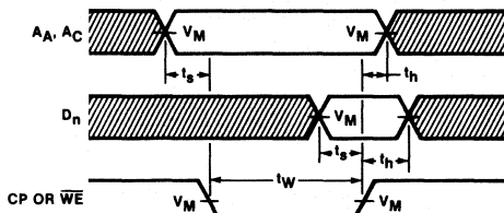
Waveform 5
