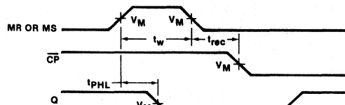
Waveform 2
