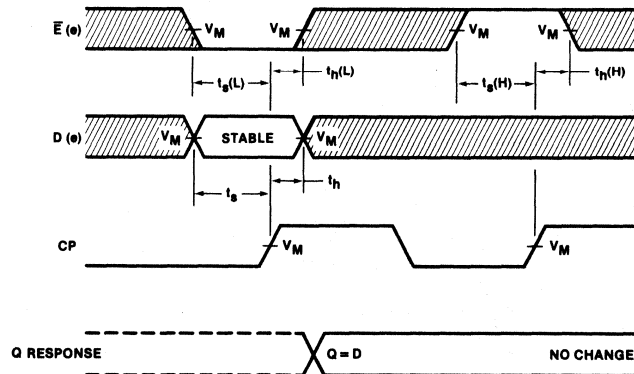
Waveform 5
