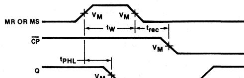
Waveform 2
