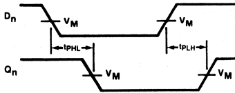
Waveform 1
