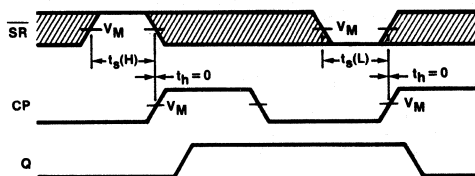
Waveform 11
