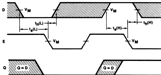
Waveform 5
