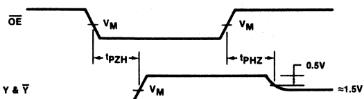
Waveform 3
