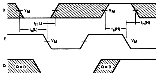
Waveform 5
