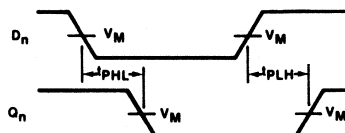
Waveform 4
