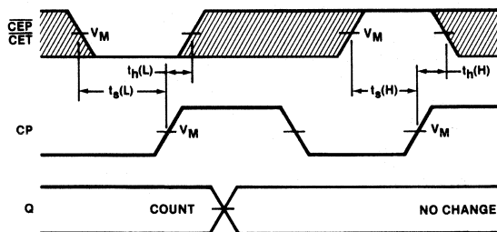
Waveform 9
