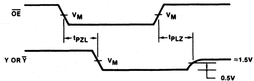
Waveform 4
