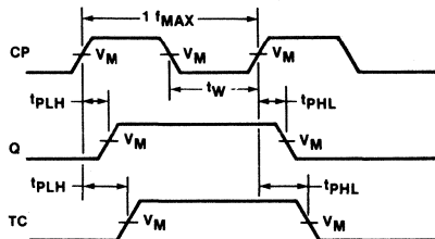
Waveform 1
