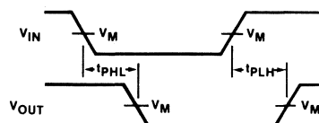
Waveform 2
