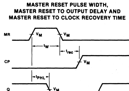
Waveform 4
