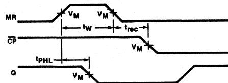
Waveform 2
