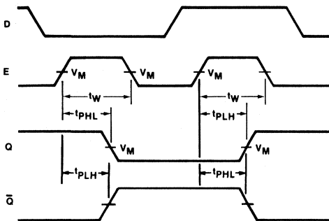
Waveform 3
