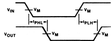
Waveform 1
