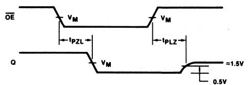
Waveform 4
