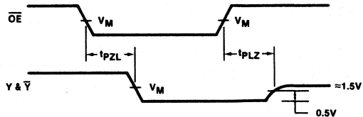
Waveform 4
