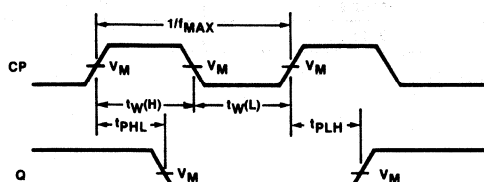
Waveform 3
