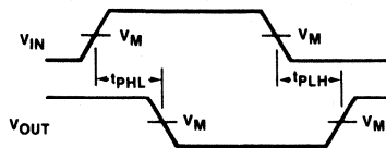
Waveform 1
