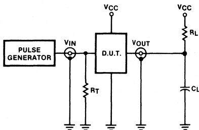
TEST CIRCUIT FOR 54/74 OPEN COLLECTOR OUTPUTS
