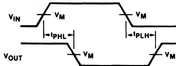
Waveform 1
