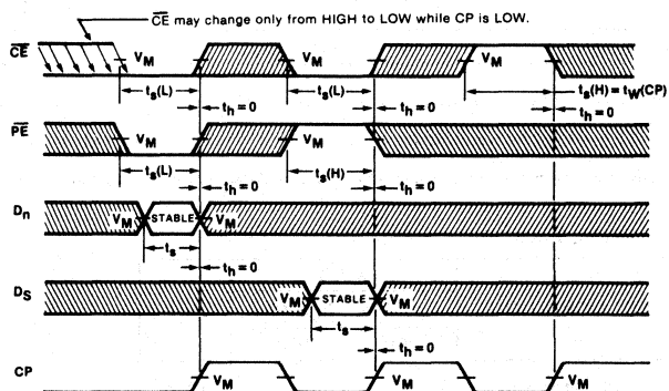
Waveform 1
