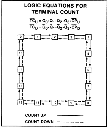
STATE DIAGRAM, '193
