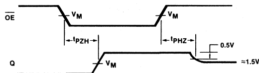
Waveform 6
