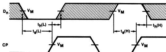
Waveform 7
