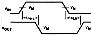
Waveform 1
