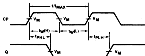
Waveform 6
