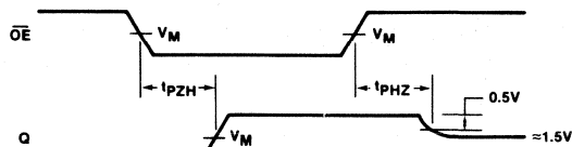
Waveform 2
