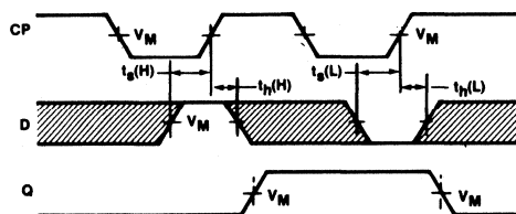
Waveform 3
