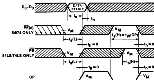
Waveform 5
