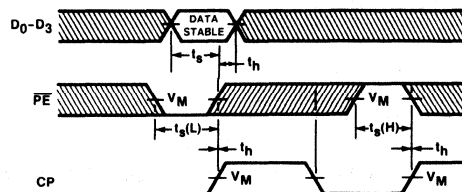
Waveform 4
