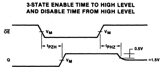
Waveform 2
