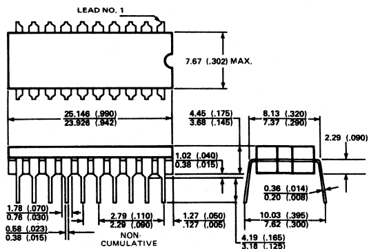
F PACKAGE CERAMIC (20-PIN DIP)
