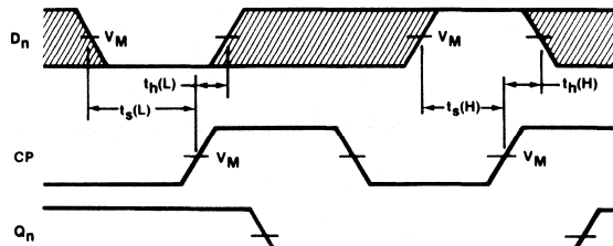
Waveform 4
