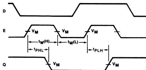
Waveform 1
