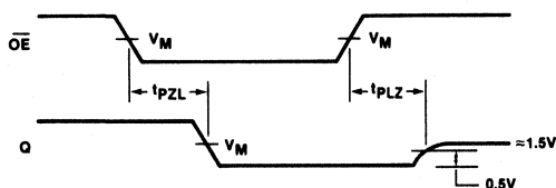
Waveform 3
