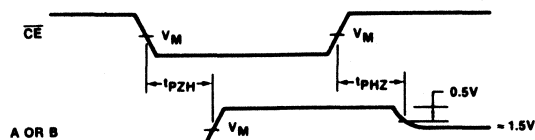
Waveform 2
