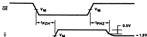
3-STATE ENABLE TIME TO HIGH LEVEL AND DISABLE TIME FROM HIGH LEVEL
