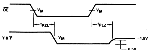
Waveform 4
