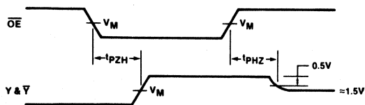
Waveform 3
