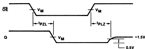
Waveform 3
