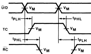
Waveform 7
