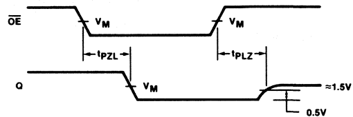
Waveform 4
