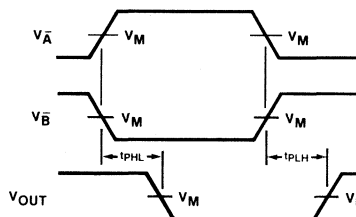
Waveform 4
