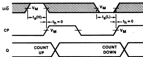
Waveform 10
