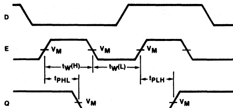
Waveform 1
