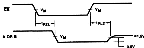
Waveform 3
