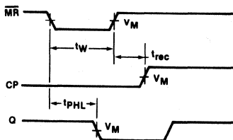
Waveform 3
