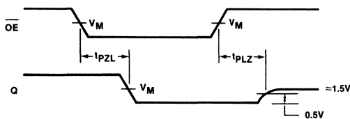
Waveform 7
