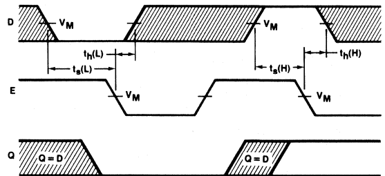
DATA SETUP AND HOLD TIMES
