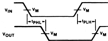
Waveform 1
