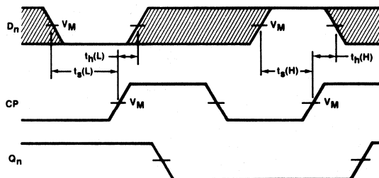
Waveform 7
