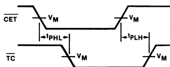
Waveform 3
