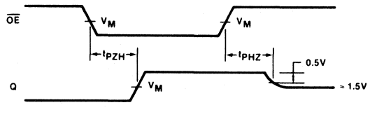
Waveform 2
