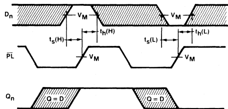
Waveform 6
