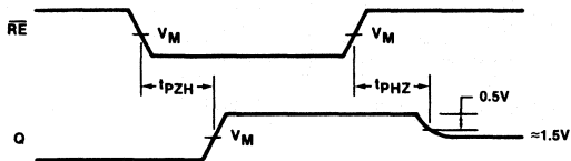
Waveform 3
