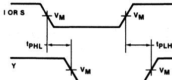
Waveform 1
