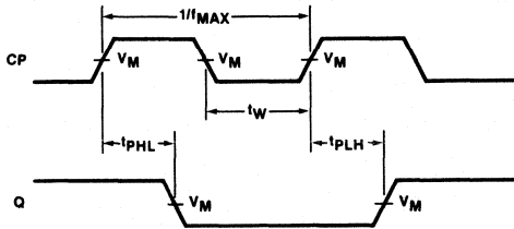
Waveform 1
