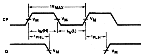
Waveform 6
