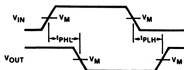
Waveform 1
