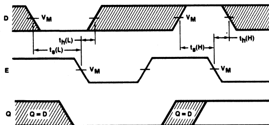
Waveform 5
