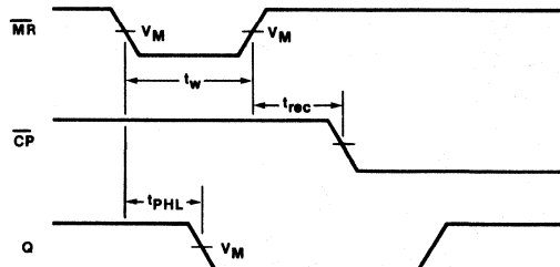
Waveform 2
