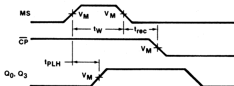
Waveform 3
