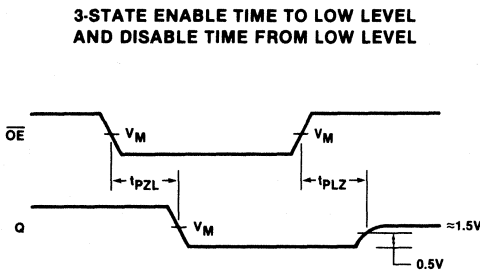
Waveform 1
