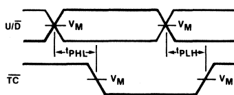
Waveform 3
