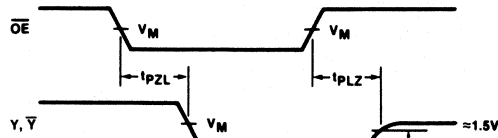
Waveform 4
