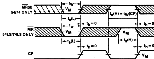
Waveform 6
