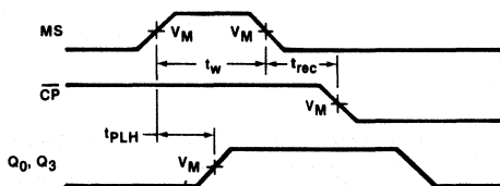
Waveform 3
