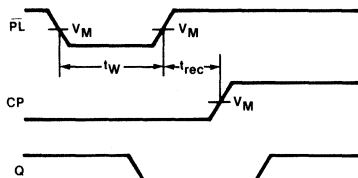
Waveform 5
