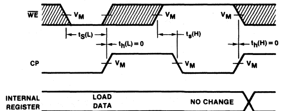
Waveform 6
