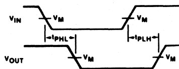
Waveform 1
