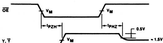
Waveform 3
