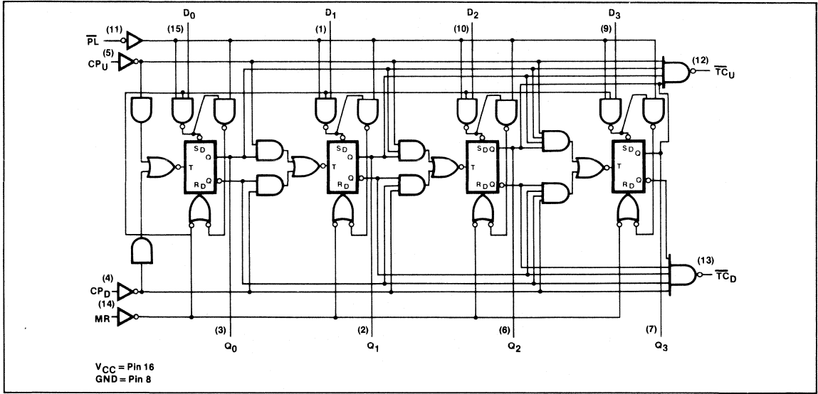
LOGIC DIAGRAM, '193
