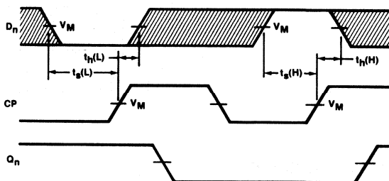
Waveform 4
