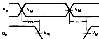
Waveform 3
