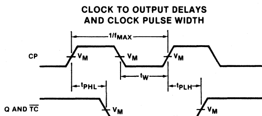
Waveform 1
