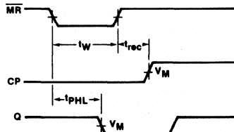
Waveform 2
