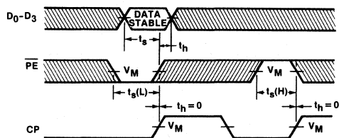
Waveform 8
