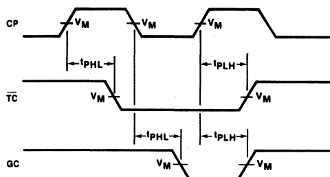
Waveform 2
