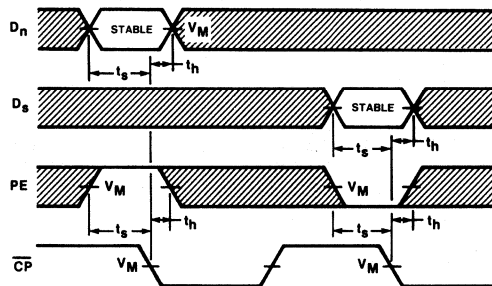
Waveform 5
