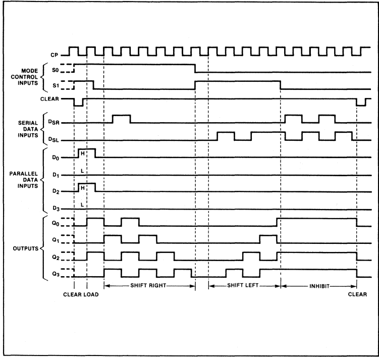
TYPICAL CLEAR, LOAD, RIGHT-SHIFT, LEFT-SHIFT, INHIBIT AND CLEAR SEQUENCES
