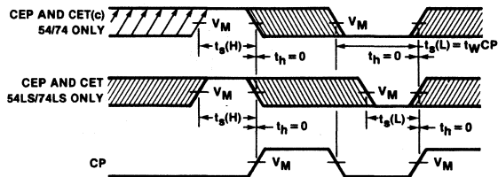
Waveform 4
