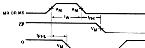
Waveform 2
