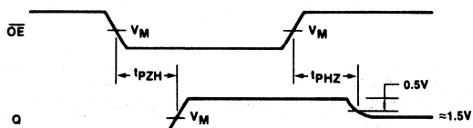
Waveform 1
