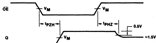
Waveform 2
