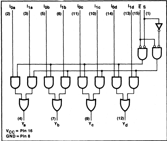
LOGIC DIAGRAM, '157
