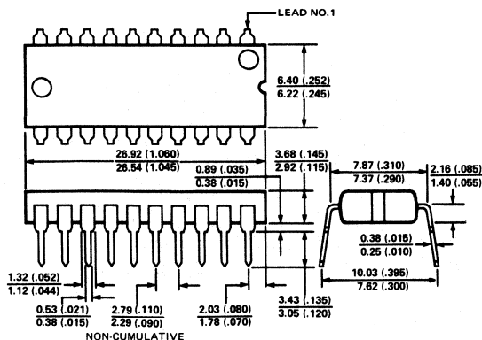
N PACKAGE PLASTIC (20-PIN DIP)
