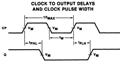
Waveform 1
