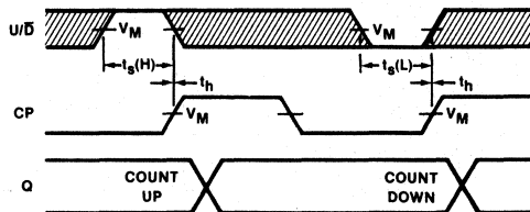
Waveform 6
