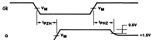
Waveform 2
