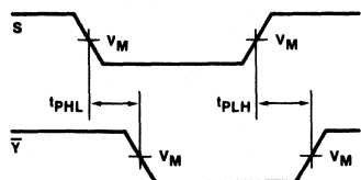
Waveform 1
