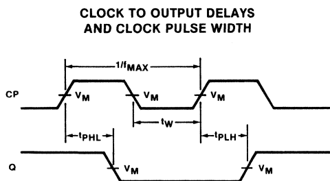
Waveform 1
