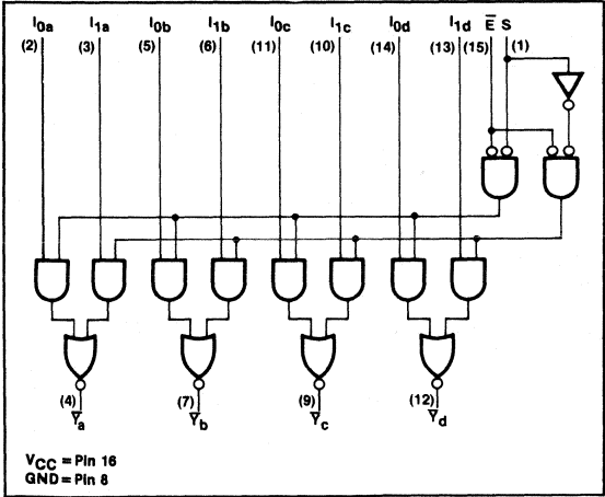
LOGIC DIAGRAM, '158
