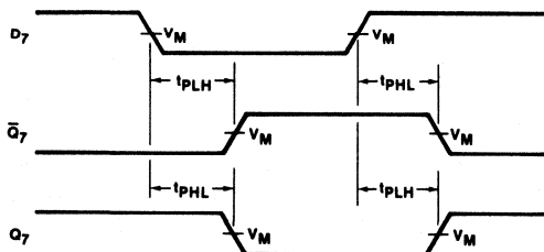
PARALLEL DATA TO OUTPUT DELAYS
