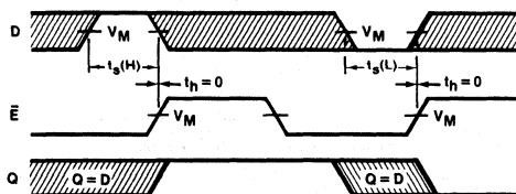
Waveform 5
