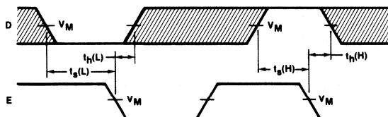
Waveform 5
