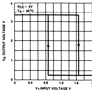
(54/74, 54LS/74LS) VIN vs VOUT TRANSFER FUNCTION
