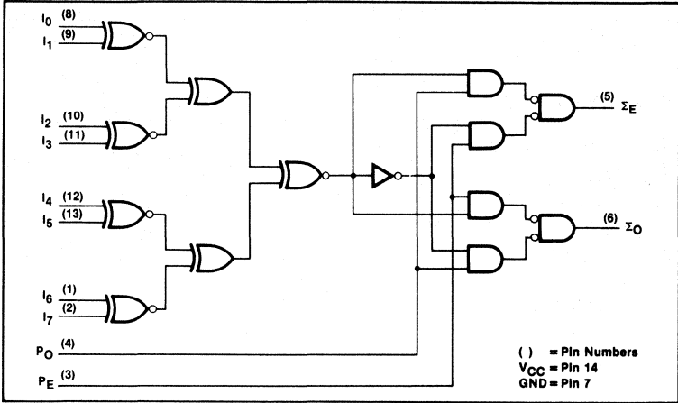
LOGIC DIAGRAM
