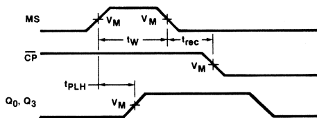
Waveform 3
