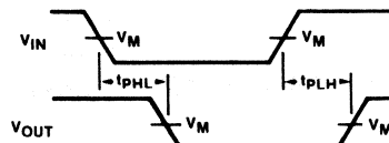
Waveform 2
