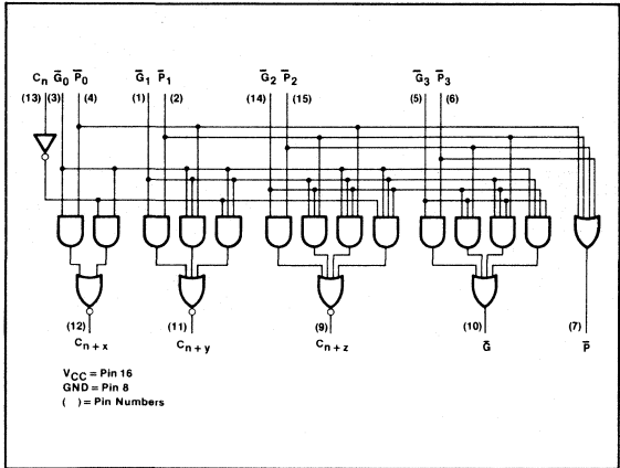
LOGIC DIAGRAM
