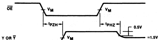
Waveform 3
