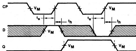
Waveform 2
