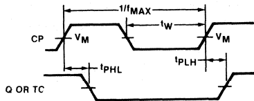
Waveform 1
