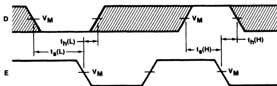
Waveform 5
