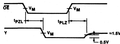
Waveform 3
