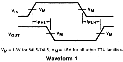
WAVEFORM FOR INVERTING OUTPUTS
